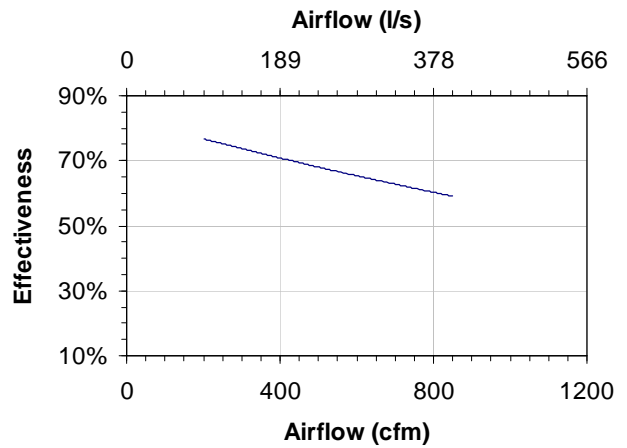
Thermal Effectiveness
