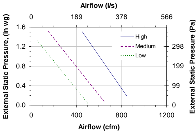
Airflow Performance
