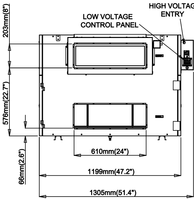
LEFT VIEW
